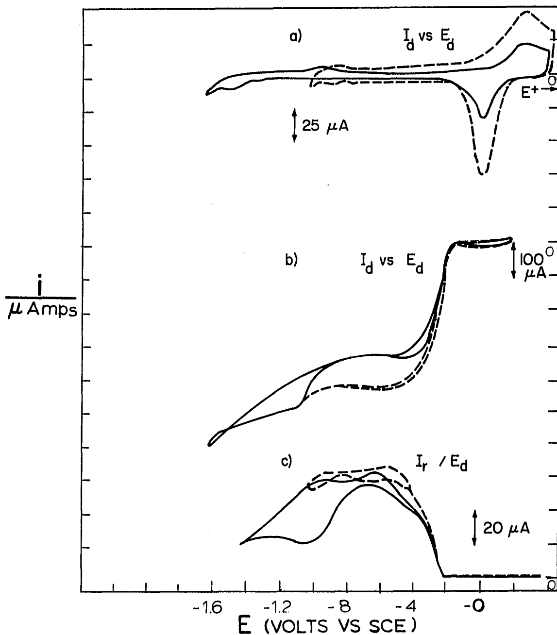
Figure IV-9. I/E data for oxygen reduction on gold electrodes in 1 M NaOH: (a) disk current for a N_2 saturated solution, (b) disk current for oxygen saturated solution, (c) ring current in an oxygen saturated solution; (---) solid gold RRDE, (—) gold plated GPE
