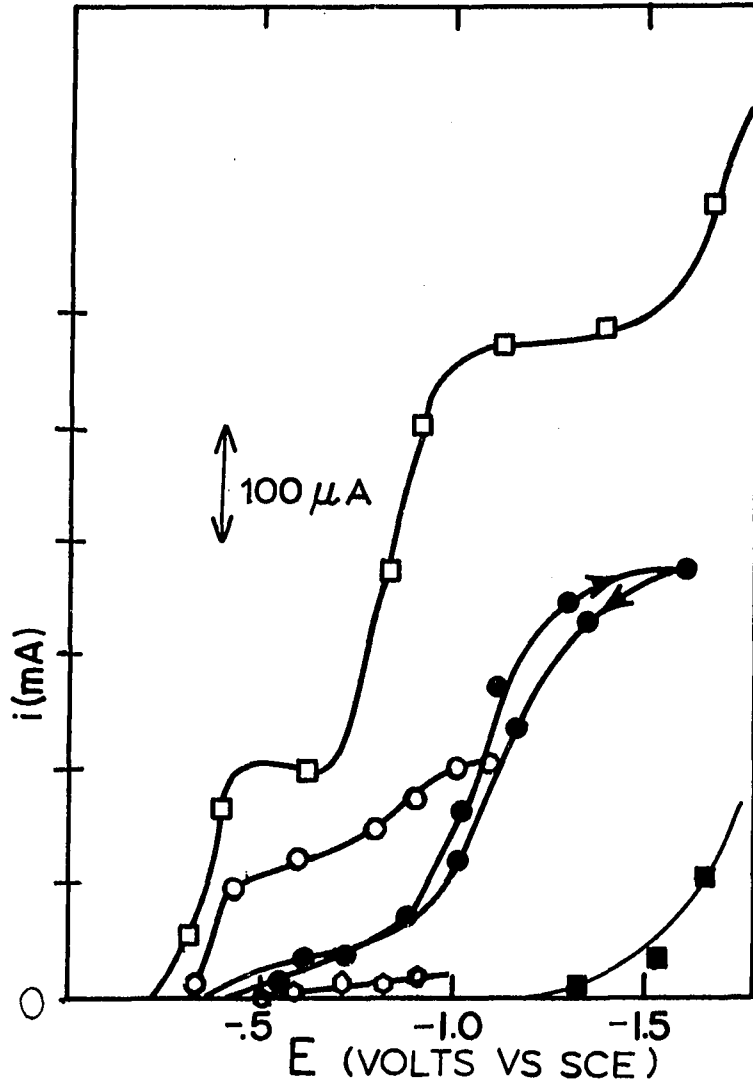
Figure IV-7. I/E wave for oxygen reduction on different carbon electrodes: (□) Taylor and Humffray (35), (o) Brezina and Hofmanova-Matejkova (93), (◐) Morcos and Yeager (38), (●) present work. (■) Results for peroxide reduction on a graphite electrode (35)
