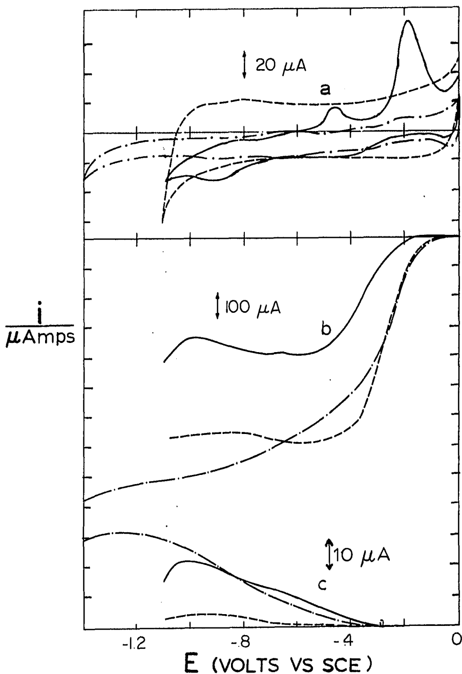
Figure IV-12. I/E scans for oxygen reduction on silver electrodes: (a) disk current in a N_2 saturated solution, (b) disk current in an O_2 saturated solution, and (c) ring current in an oxygen saturated solution; (---) solid silver RRDE, (—) silver plated GPE, (-·-·) reduced silver GPE
