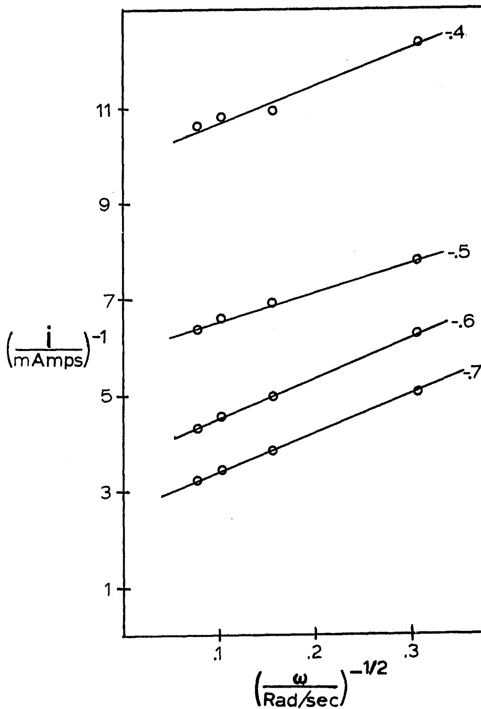
Figure IV-17. 1/i_d versus \omega^{-1/2} for oxygen reduction on a reduced platinum GPE
