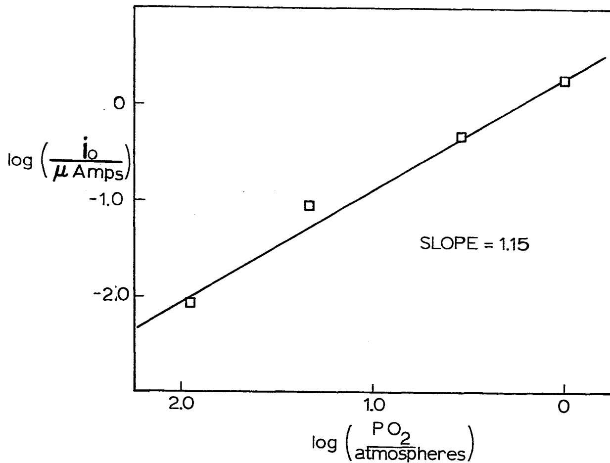
Figure IV-6. \log i_0 is plotted against the log of oxygen partial pressure for oxygen reduction in 1 M NaOH on a GPE.
